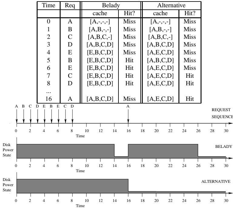
Figure 3: An example showing that Belady’s algorithm is not energy-optimal.
