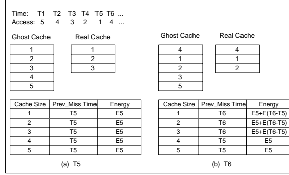
Figure 6: An example of energy estimate in PB-LRU for a disk
