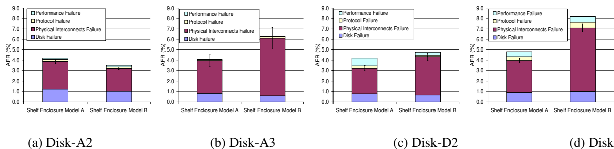
Figure 6. AFR for storage subsystems of low-end storage systems by shelf enclosure models using the same disk models (a subset of data from Figure 5). The error bars show 99.5%+ confidence intervals for physical interconnect failures.
